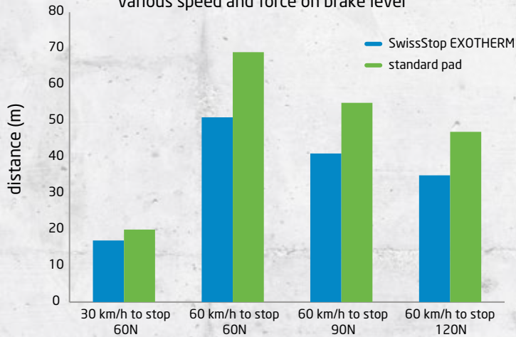
STOPPING DISTANCES various speed and force on brake lever
